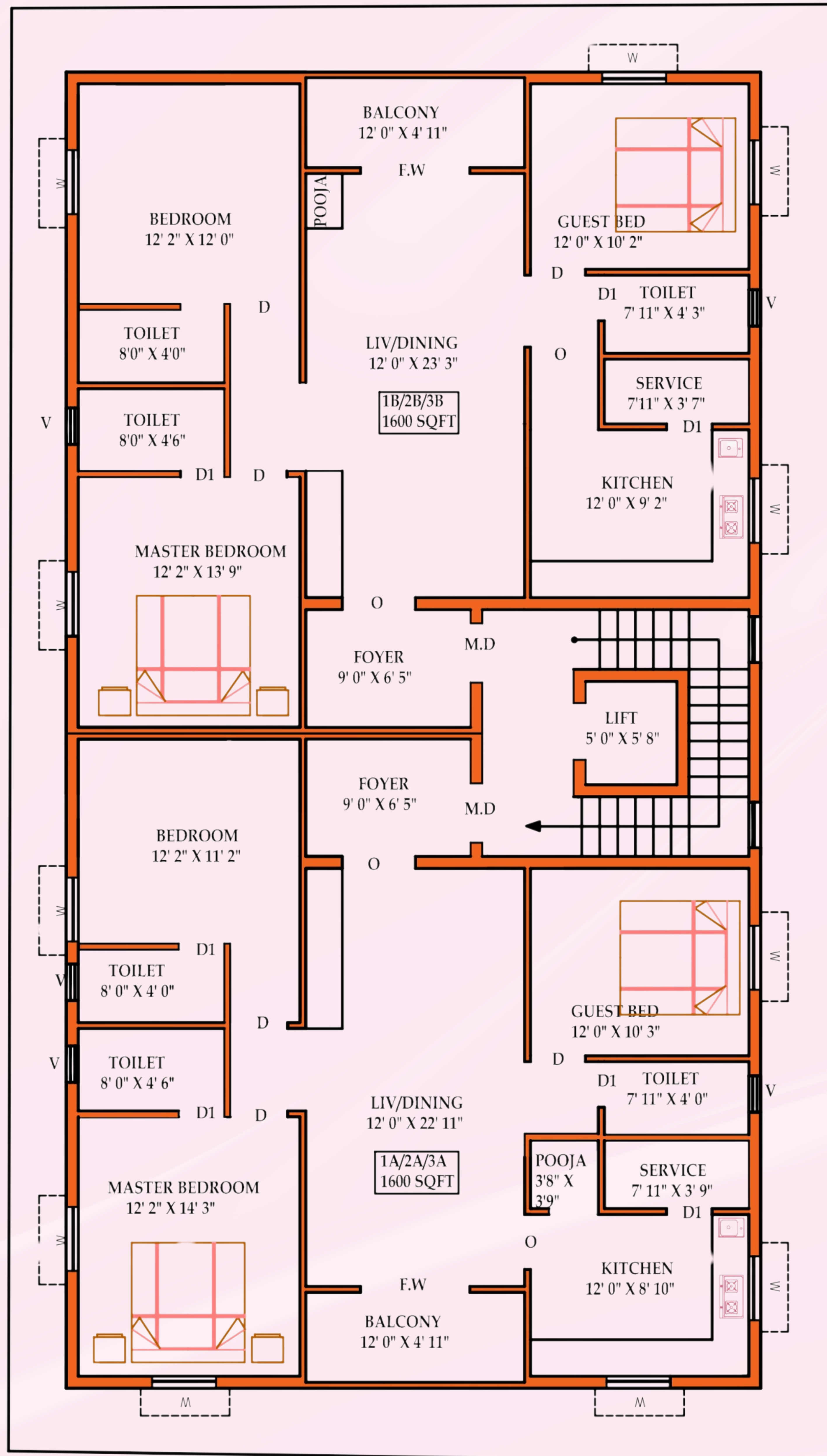
TYPICAL 1,2&3 FLOOR PLAN
