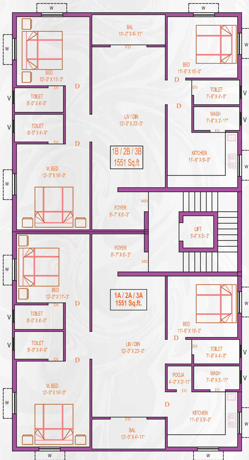
TYPICAL 1, 2 & 3 FLOOR PLAN
